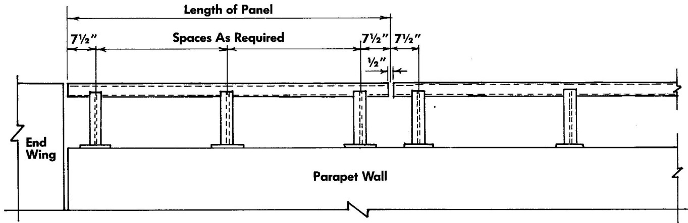
Typical Rail Detail
