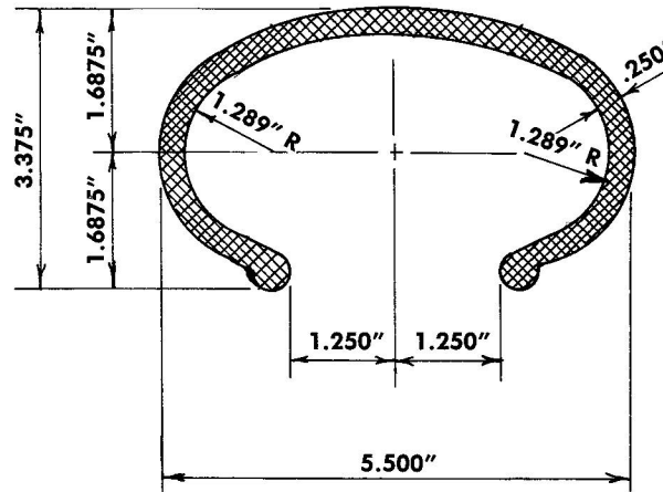
Rail Member Die #11136-B
