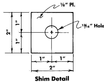
Shim Detail
