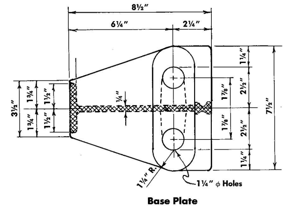
Base Plate
